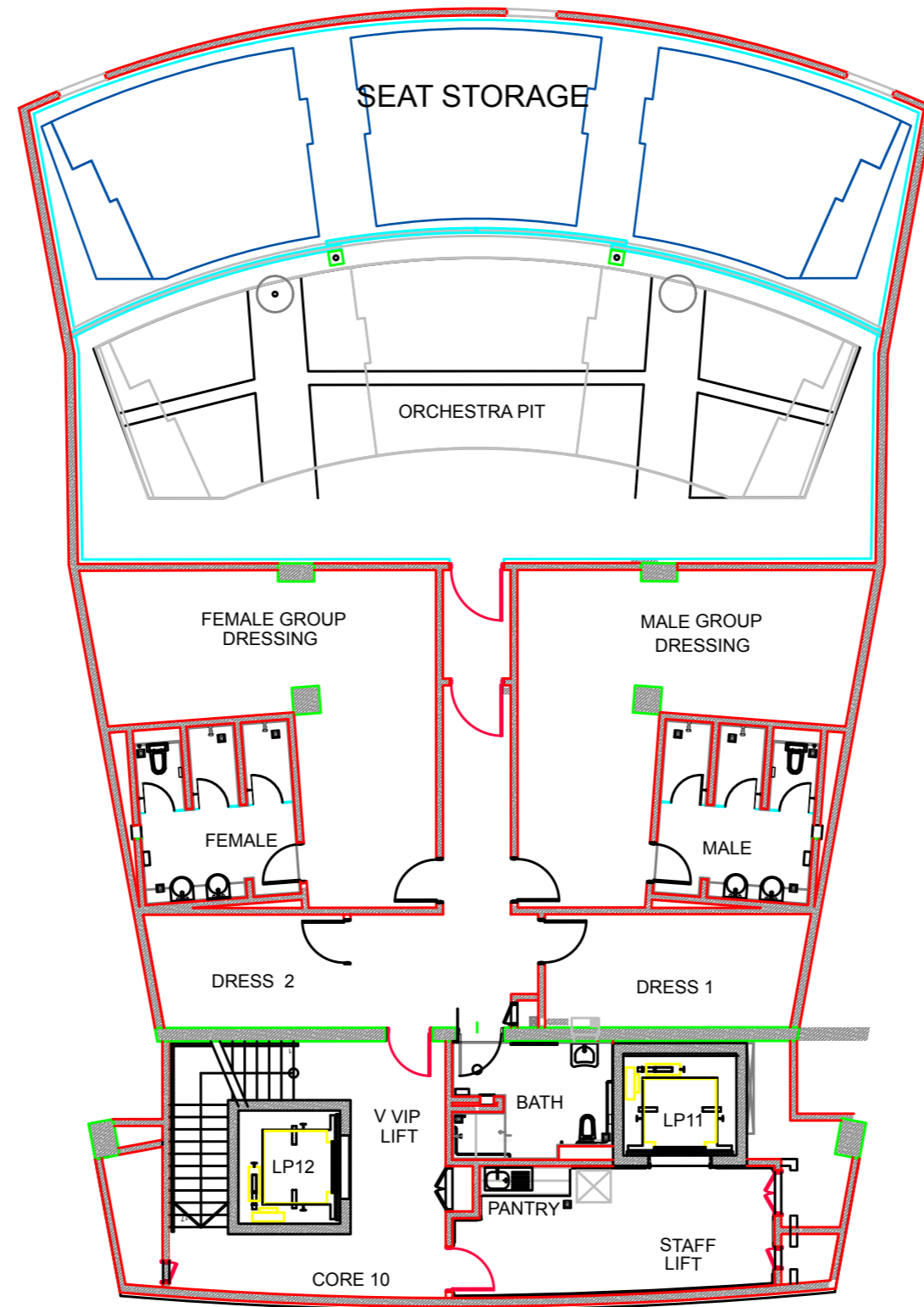
PLENARY HALL MEZZANINE FLOOR PLAN
