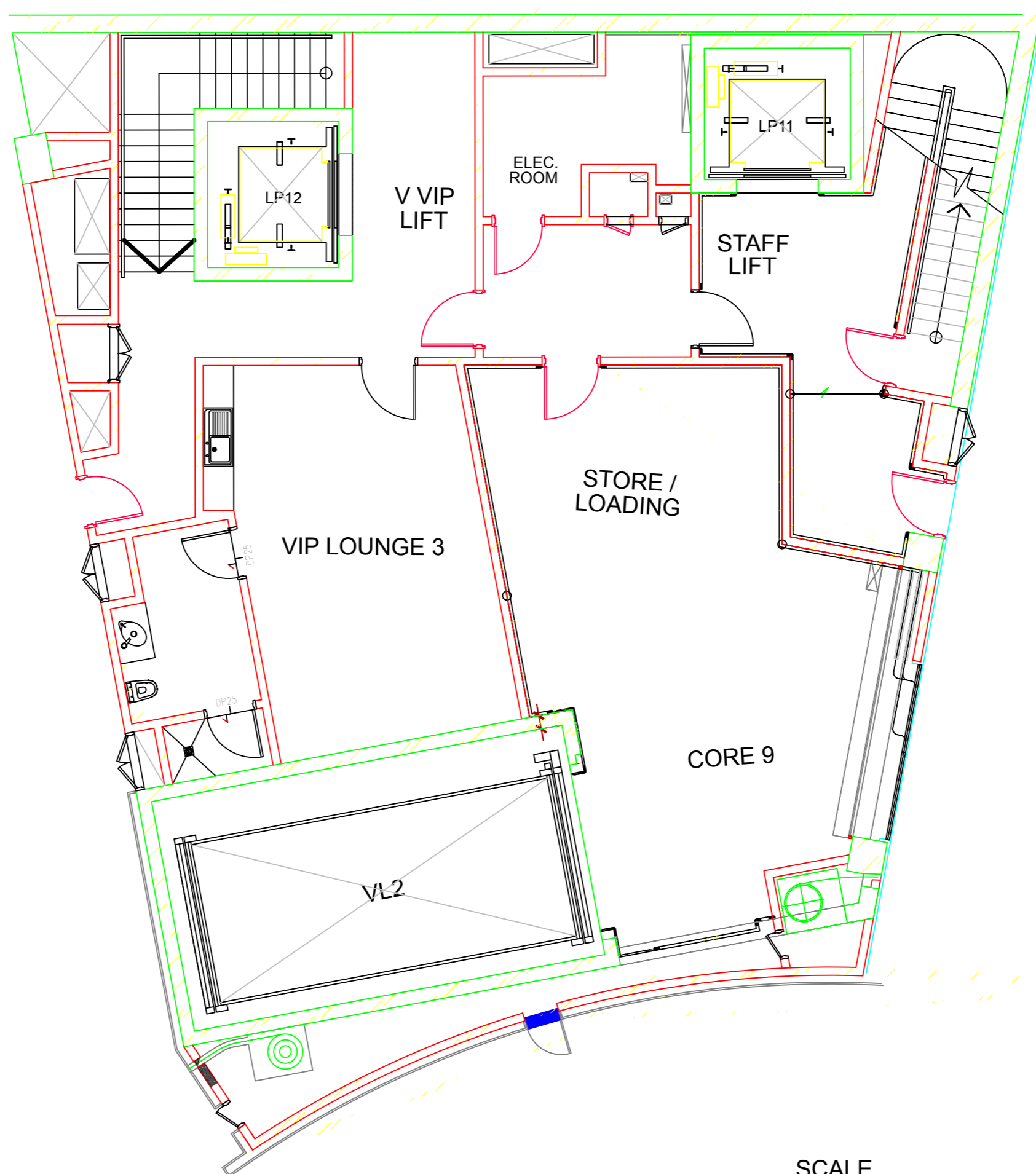
PLENARY HALL-VIP LOUNGE 3RD FLOOR PLAN
